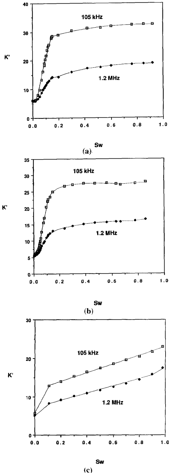
FIG. 1. K' versus S_w for the three sandstones at two frequencies, 105 kHz and 1.2 MHz. (a) CH61-79, (b) CH58-79, (c) Berea 100.
