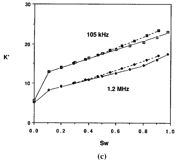
FIG. 6. Comparison of data for the three sandstones with CRIM for the wetted rock, bulk water, air system. Data are open symbols connected with a solid line; CRIM results are solid symbols connected with a broken line. (a) CH61-79; (b) CH58-79; (c) Berea 100.
