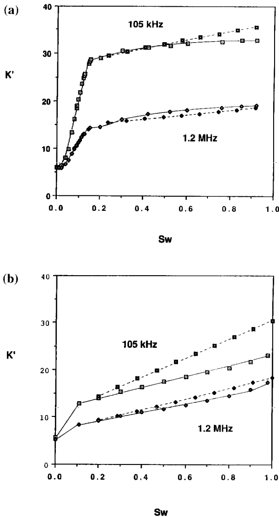
FIG. 8. Comparison of data with results from effective medium theory when a complex matrix dielectric constant is used. Data are open symbols connected with a solid line; effective medium theory results are solid symbols connected with a broken line. (a) CH61-79; (b) Berea 100.
