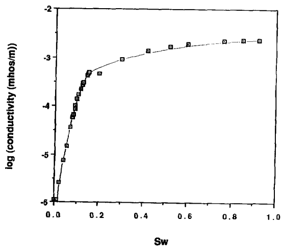
FIG. 7. Log (conductivity) versus S_w measured for CH61-79 at 105 kHz.
