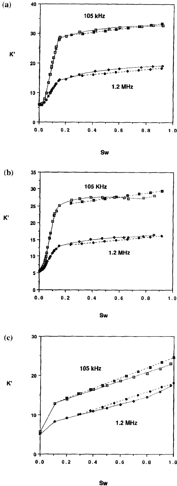
FIG. 4. Comparison of data for the three sandstones with effective medium theory for the wetted rock, bulk water, air system. Data are open symbols connected with a solid line; effective medium theory results are solid symbols connected with a broken line. (a) CH61-79; (b) CH58-79; (c) Berea 100.
